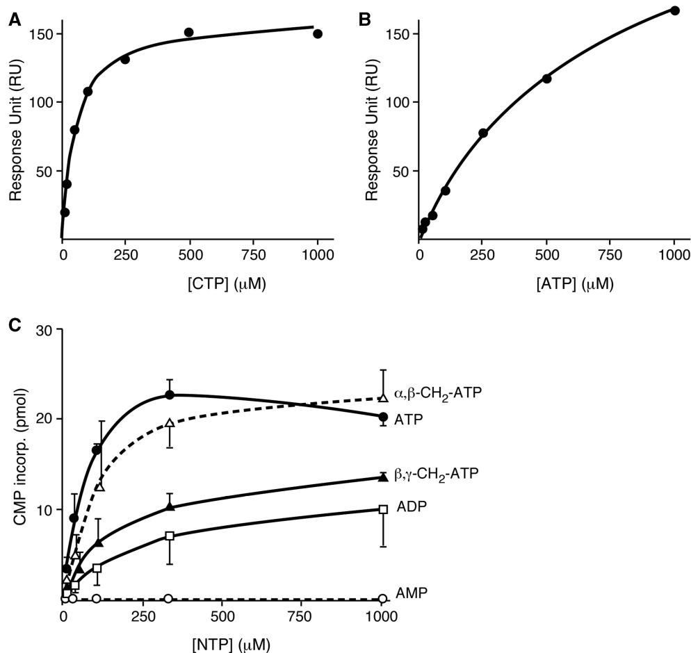
Figure 5. Effect of ATP and CTP on the binding of T7 DNA primase to its recognition sequence. Binding of the primase (10 \mu\text{M} ) to an oligonucleotide containing a recognition sequence 5'-TG \mathbf{GTC} -3' (250 RU) in the presence of various concentrations of ATP or CTP was measured by SPR assay. (A) The indicated concentration of CTP was present in the binding reaction together with 0.2 mM ATP. (B) The indicated concentration of ATP was present in the binding reaction together with 0.2 mM CTP. (C) Effect of the 5'-phosphate of ATP on primer synthesis. Primer synthesis reactions were carried out with 0.5 \mu\text{M} 25-mer ssDNA containing a recognition sequence 5'-GG \mathbf{GTC} -3', 5 \mu\text{M} T7 DNA primase, 0.2 mM [ \alpha\text{-}^{32}\text{P} ] CTP (0.1 \mu\text{Ci}/\mu\text{l} ) and various concentration of ATP or its analogs (12, 37, 111, 333 and 1000 \mu\text{M} ). After separation of reaction products by polyacrylamide gel electrophoresis, incorporation of CMP into a major product, pppACCC, was determined by phosphoimager analysis and plotted against ATP or its analog concentration. Data from three independent experiments are shown.
